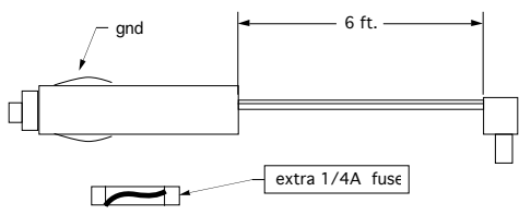
Cigarette Lighter Power Pack (pn 85058Rev0)
