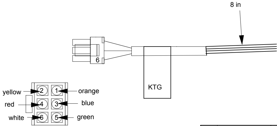
J1 REAR VIEW
