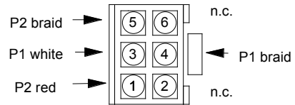
J1 REAR VIEW J1 Reference
